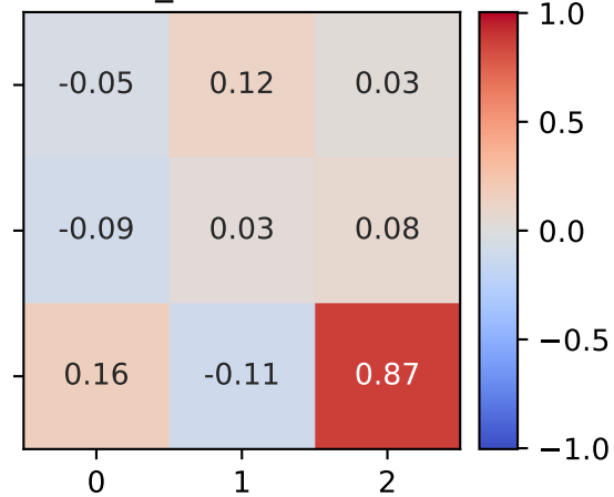
core_tensor[2, :, :]
